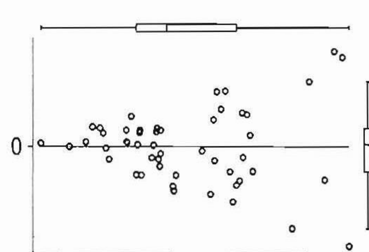
Heteroscedasticity
